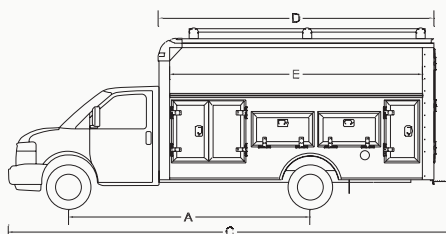
14-FT 159" WB
